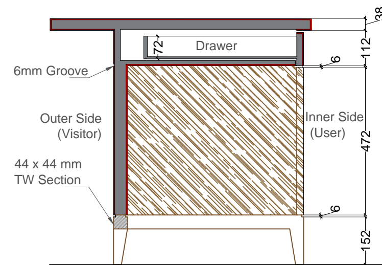
SECTION BB
