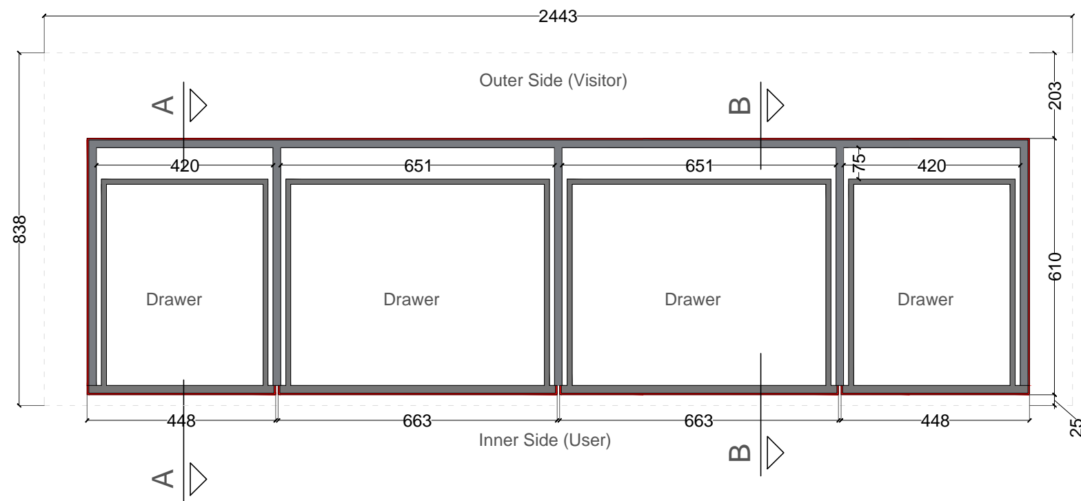
PLAN AT DRAWER LEVEL
