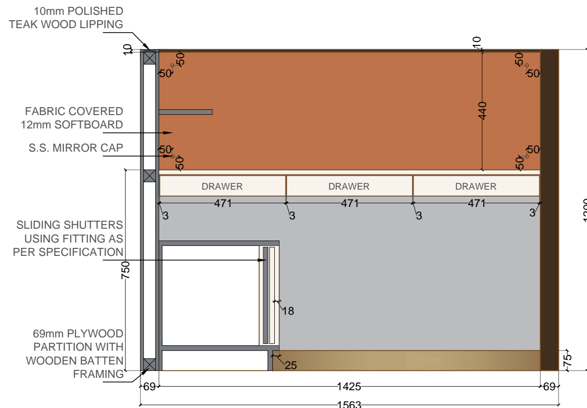
SECTIONAL ELEVATION C
