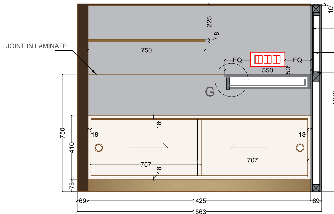
SECTIONAL ELEVATION B
