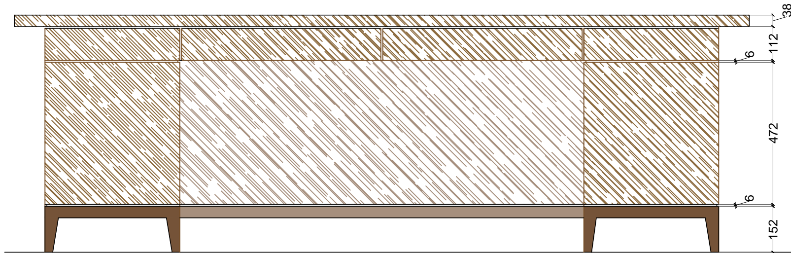
ELEVATION - In (User) Side
