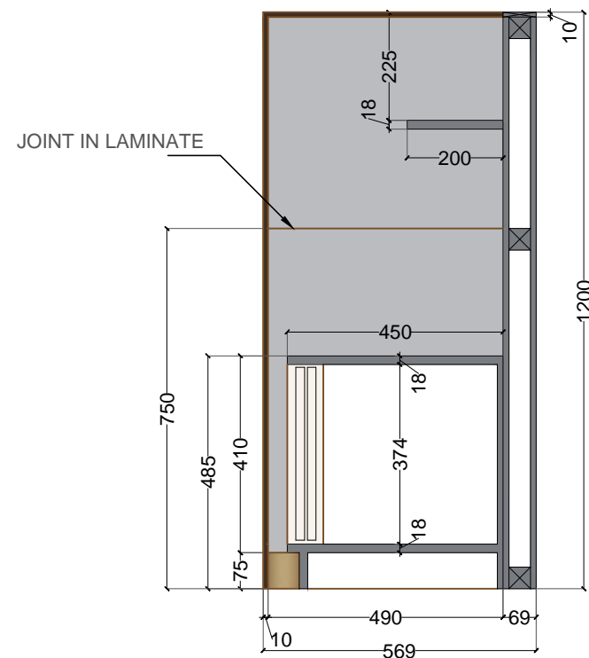
SECTIONAL ELEVATION A
