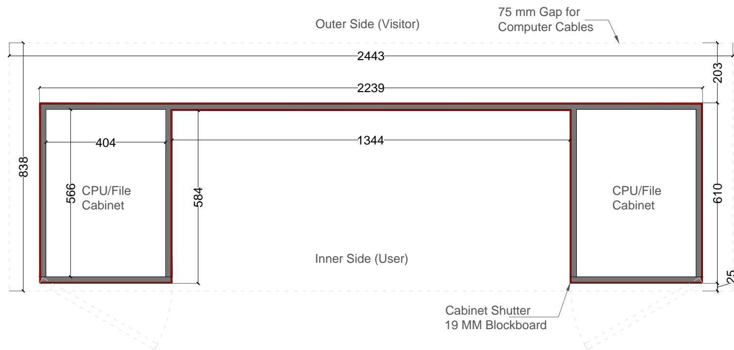
PLAN AT DRAWER LEVEL
