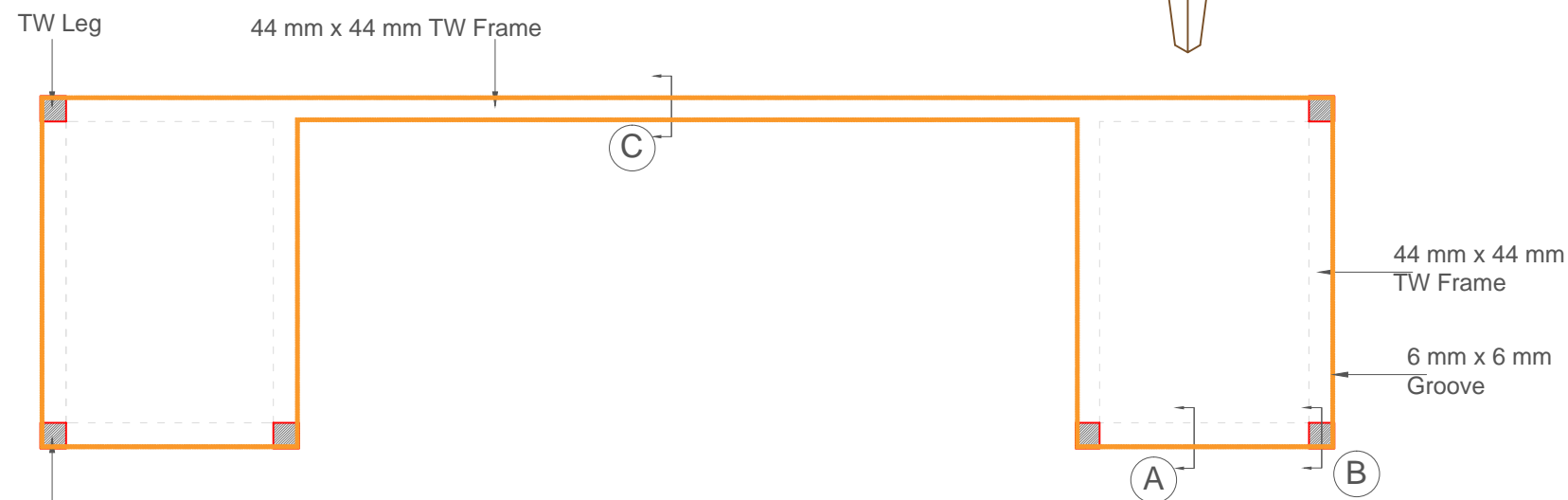
TW STAND - PLAN (FOR LEGS LOCATIONS)
