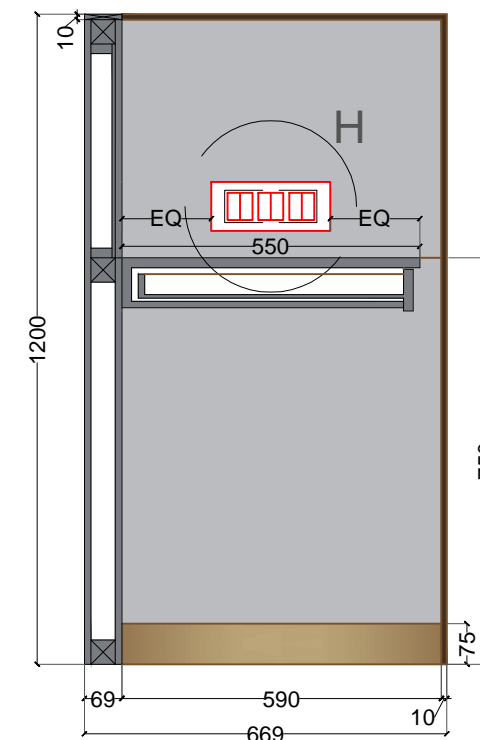
SECTIONAL ELEVATION D
