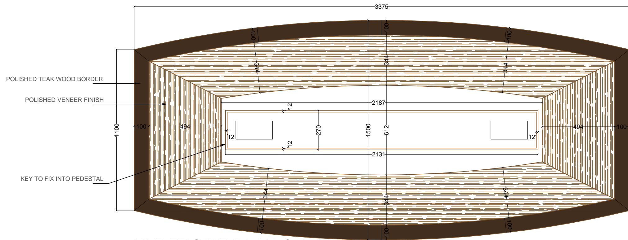
UNDERSIDE PLAN OF TABLE TOP
